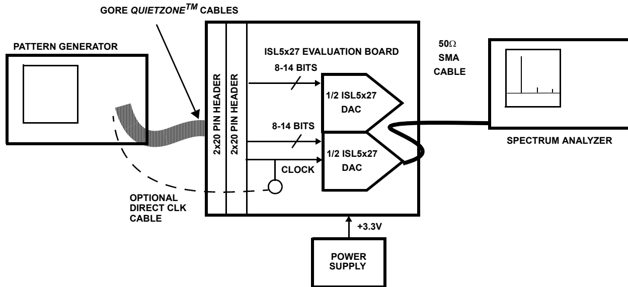
FIGURE 1. INTERSIL ISL5x27 EVALUATION SYSTEM SETUP BLOCK DIAGRAM
